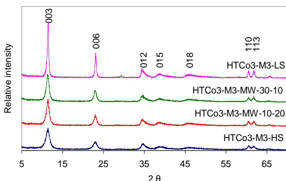
Fig. 1 XRD patterns of HTC synthesized using different methods.
