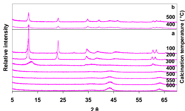
Fig.2 XRD patters of HTCo3-M3-LS: a) calcined at different temperatures; b) reconstituted after calcination at different temp.
